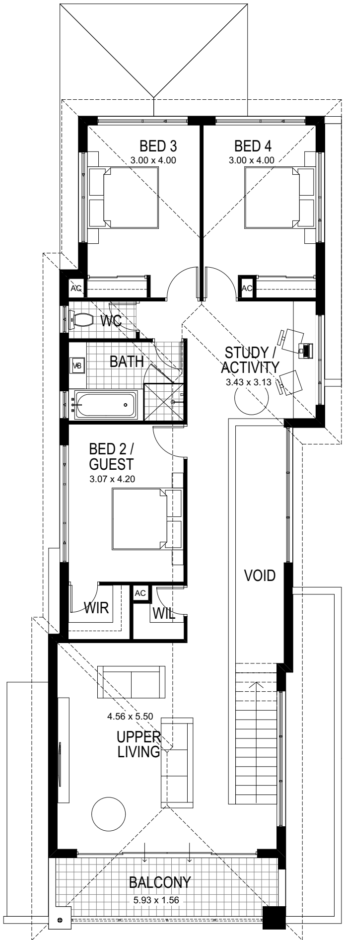
UPPER STOREY PLAN 1:100
