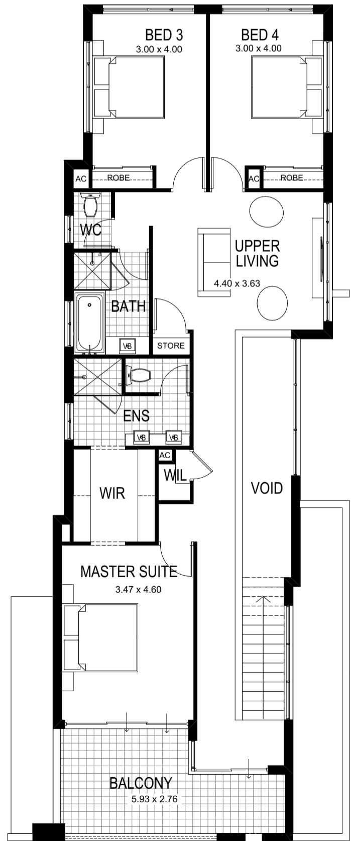
UPPER STOREY PLAN 1:100
